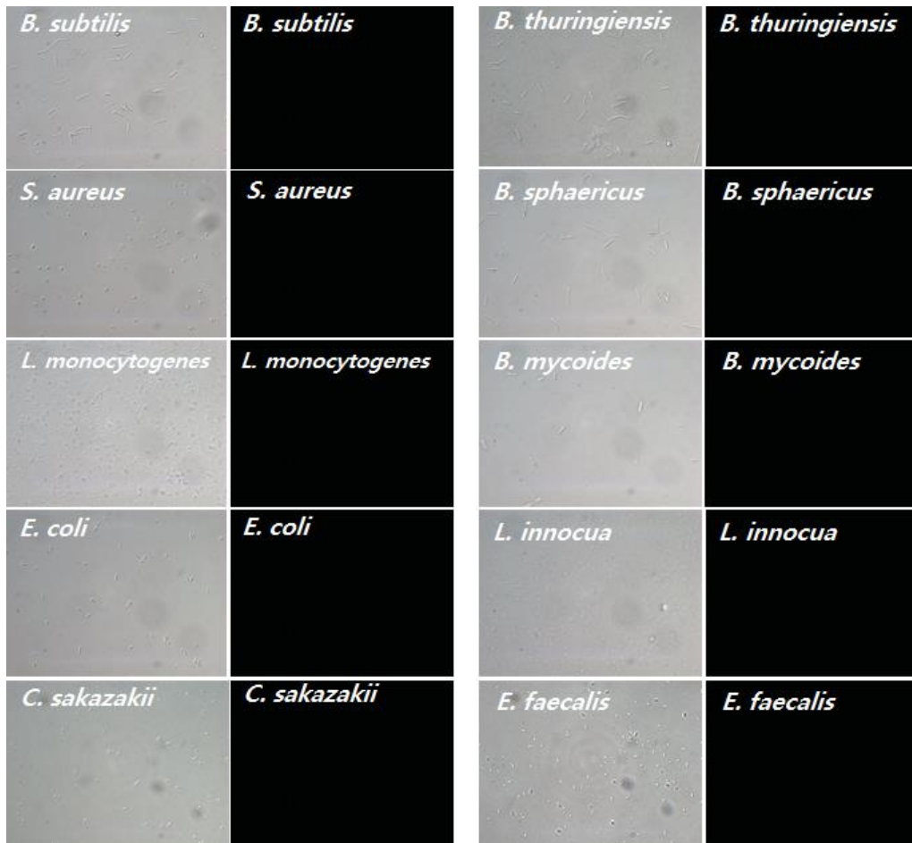
Fig. S1. Optical and fluorescent images of various bacterial species after the addition of GFP-LysPBC1_CBD.
